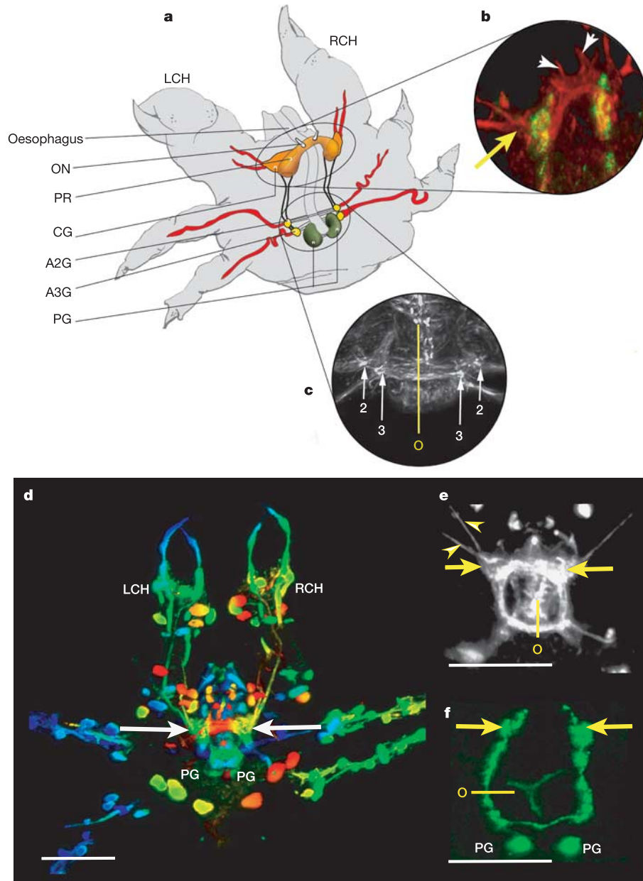
Figure 3 | CNS of the Anoplodactylus sp. larva (protonymph). a , Diagram of the protonymph seen from an oblique posteriolateral view based on reconstructions from confocal stacks ( b–f ). The CNS consists of four pairs of ganglia connected by commissures across the midline. The oesophagus runs through the proboscis between the left (LCH) and right (RCH) chelifore, and ends incompletely at the posterior ganglia (PG). The first neuromere is the protocerebrum, consisting of anteriolateral cheliforal ganglia (CG) connected by a prominent supraoesophageal protocerebral commissure (PR), and ocular nerves (ON). b , High magnification of the protocerebrum stained for tubulin (red) and serotonin (green) showing the cheliforal ganglion (arrows) and bifurcating ocular nerves ( b , arrowheads). Circumoesophageal connectives run posteriorly from the PR, leading to the second (A2G) and third (A3G) ganglia that innervate the second and third
