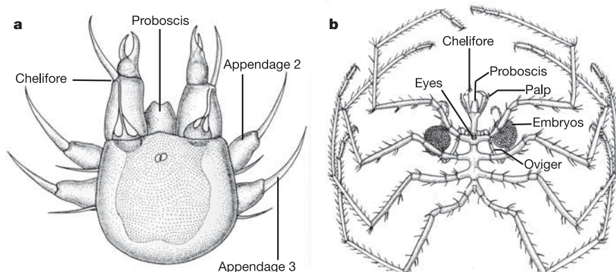
Figure 2 | The unique adult and larval morphology of pycnogonids. a , The three appendages of the protonymph larva (shown) correspond to the cephalic appendages of the adult pycnogonid. (Modified from ref. 26.) b , The
