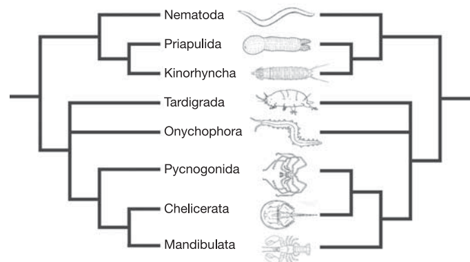
Figure 1 | Proposed relationships of pycnogonids among other ecdysozoans. The tree to the left reflects the Cormogonida hypothesis, with Pycnogonida as sister group to remaining extant arthropods. The tree to the right reflects the classical hypothesis of pycnogonids as sister group to chelicerates.
